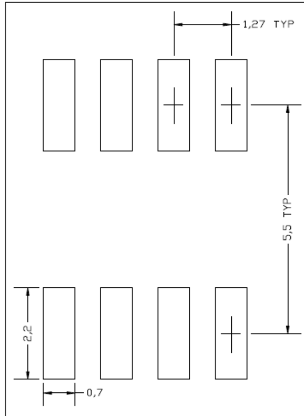
8-Pin SOIC
